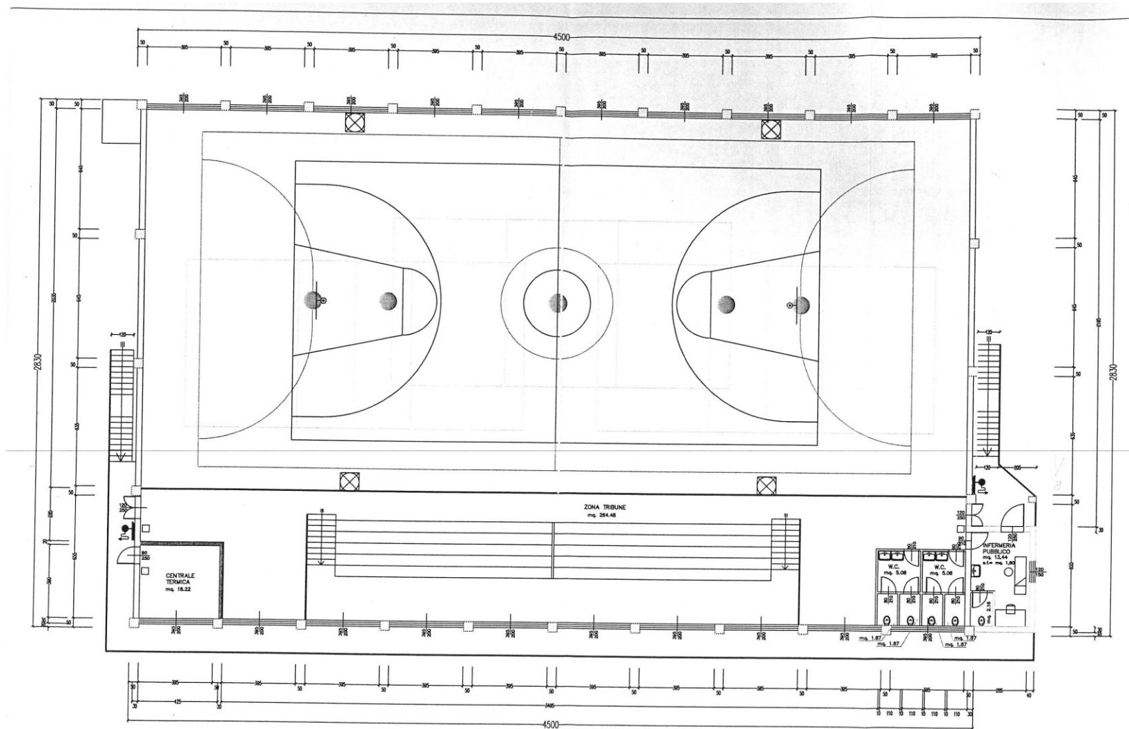
PIANTA PIANO TRIBUNE
